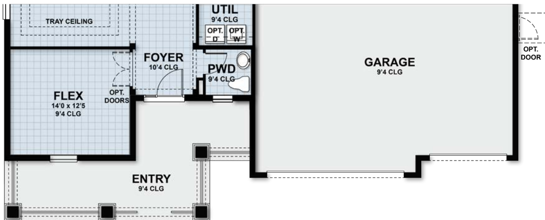
FIRST FLOOR D
